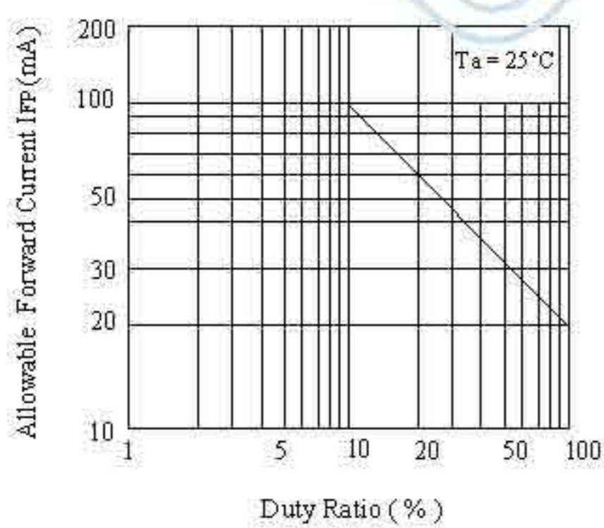
Duty Ratio vs. Allowable Forward Current
