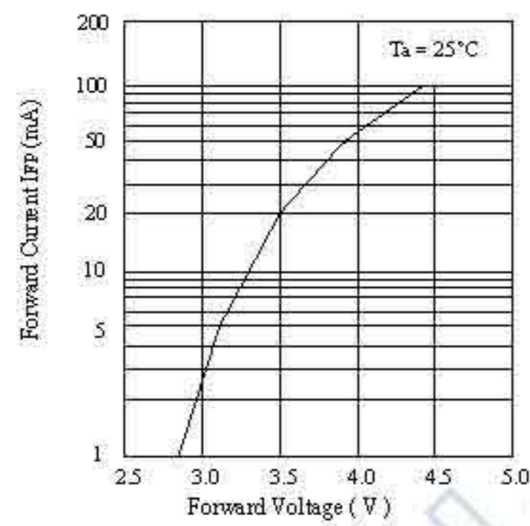
Forward Voltage vs. Forward Current
