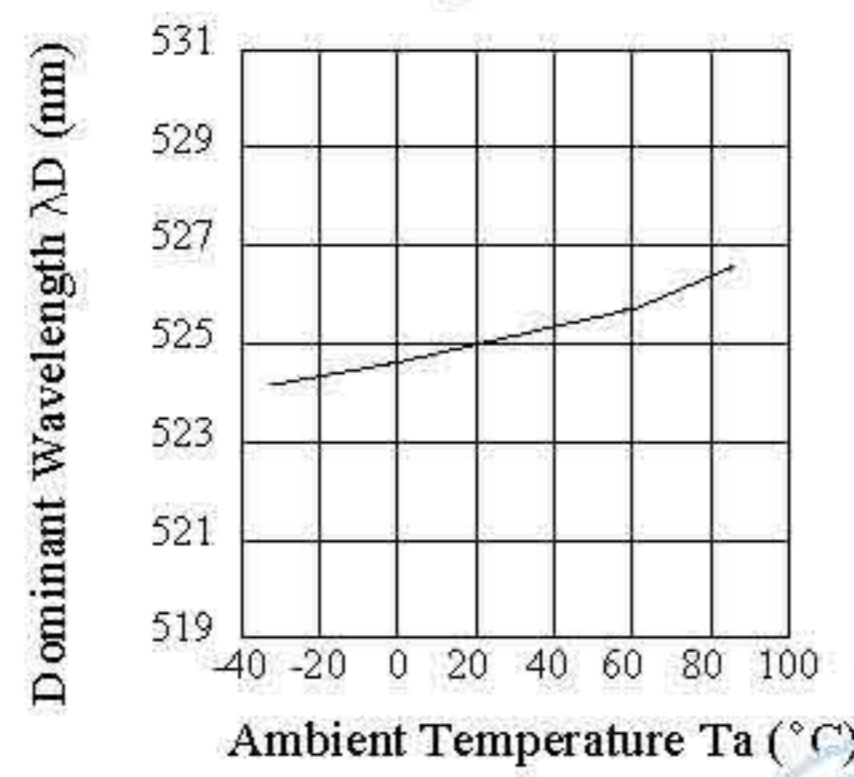
Ambient Temperature vs. Dominant Wavelength
