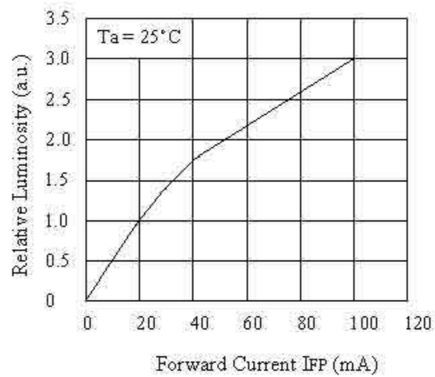
Forward Current vs. Relative Luminosity
