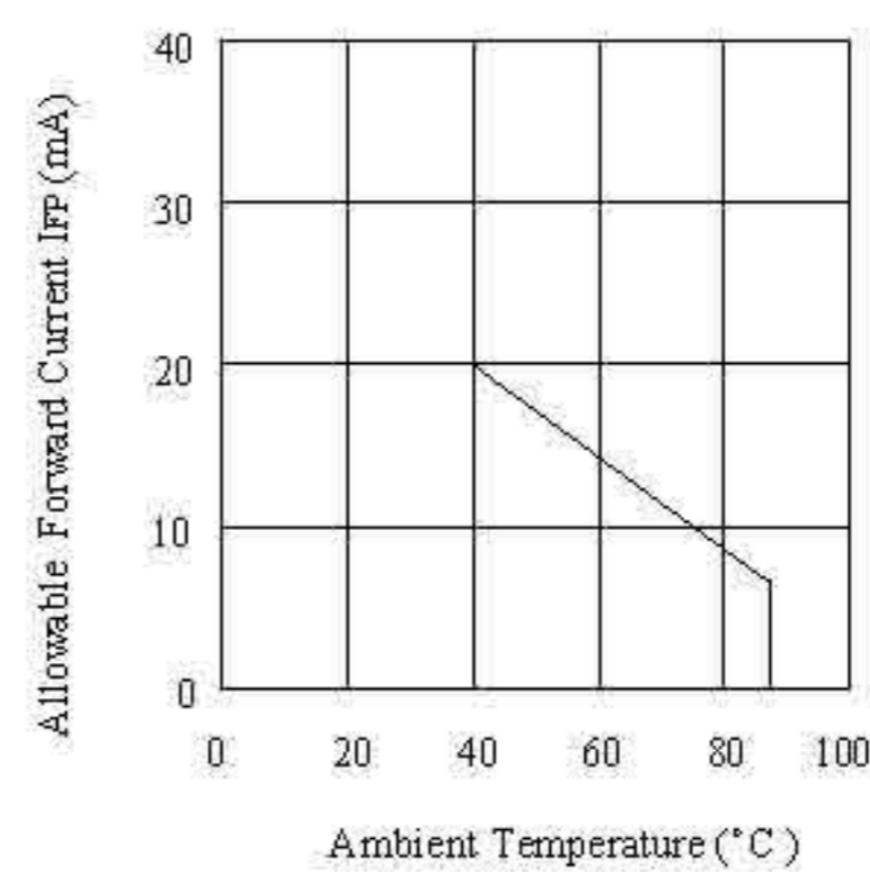
Ambient Temperature vs. Allowable Forward Current
